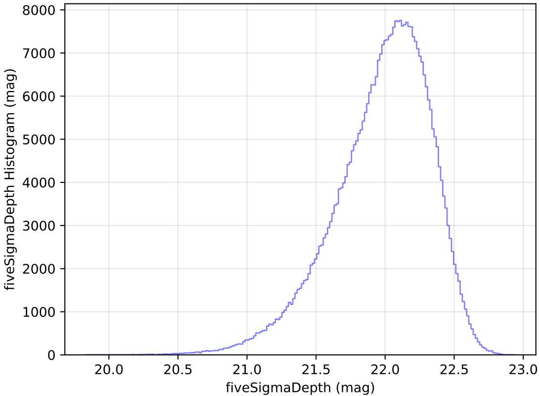
too_elab_r8_d3_giz_v3.4_10yrs y: fiveSigmaDepth Histogram
