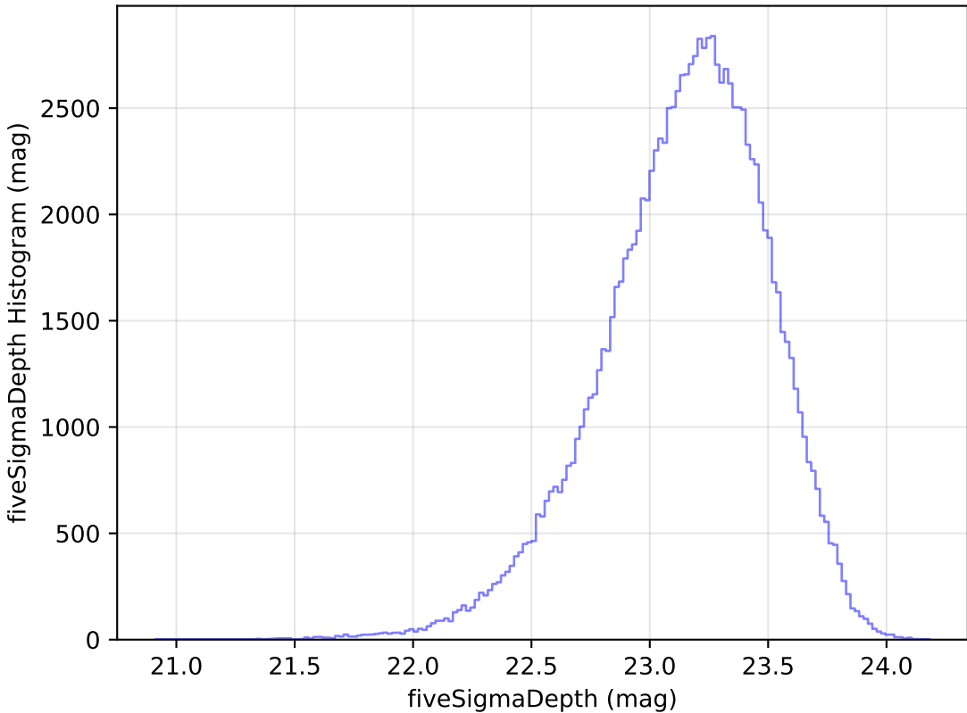
too_elab_r8_d3_giz_v3.4_10yrs u: fiveSigmaDepth Histogram
