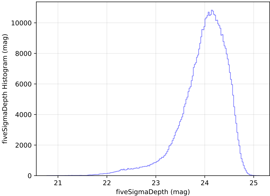
too_elab_r8_d3_giz_v3.4_10yrs r: fiveSigmaDepth Histogram
