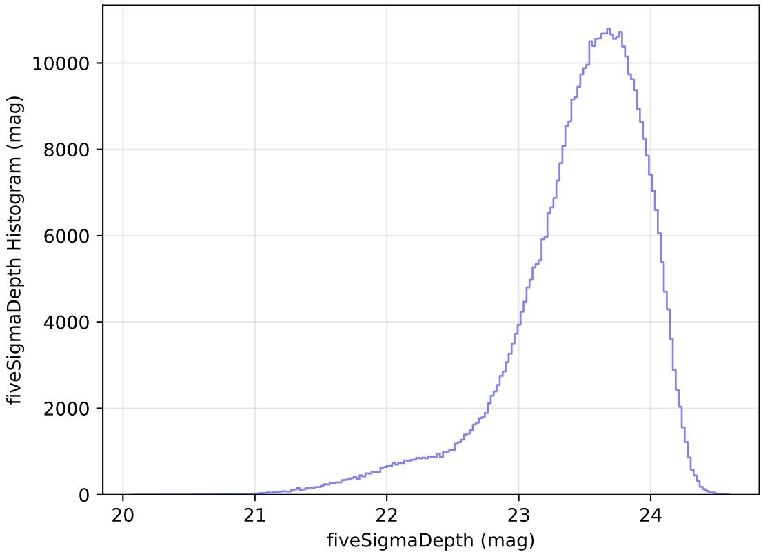
too_elab_r8_d3_giz_v3.4_10yrs i: fiveSigmaDepth Histogram
