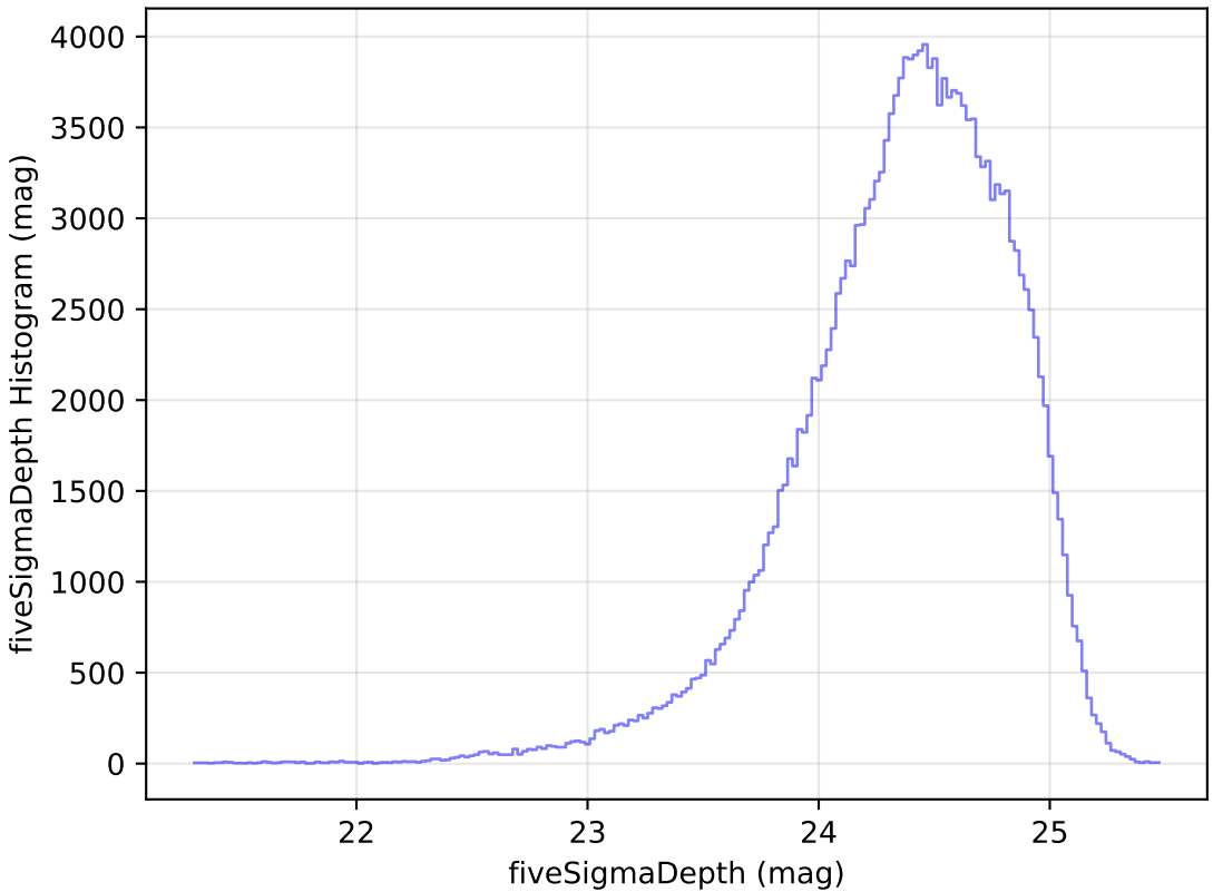
too_elab_r8_d3_giz_v3.4_10yrs g: fiveSigmaDepth Histogram
