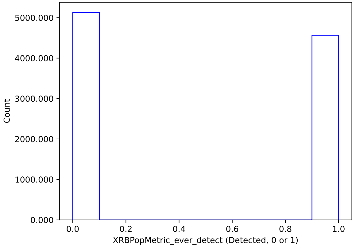
too_elab_r8_d3_giz_v3.4_10yrs : XRBPoMetric_ever_detect
