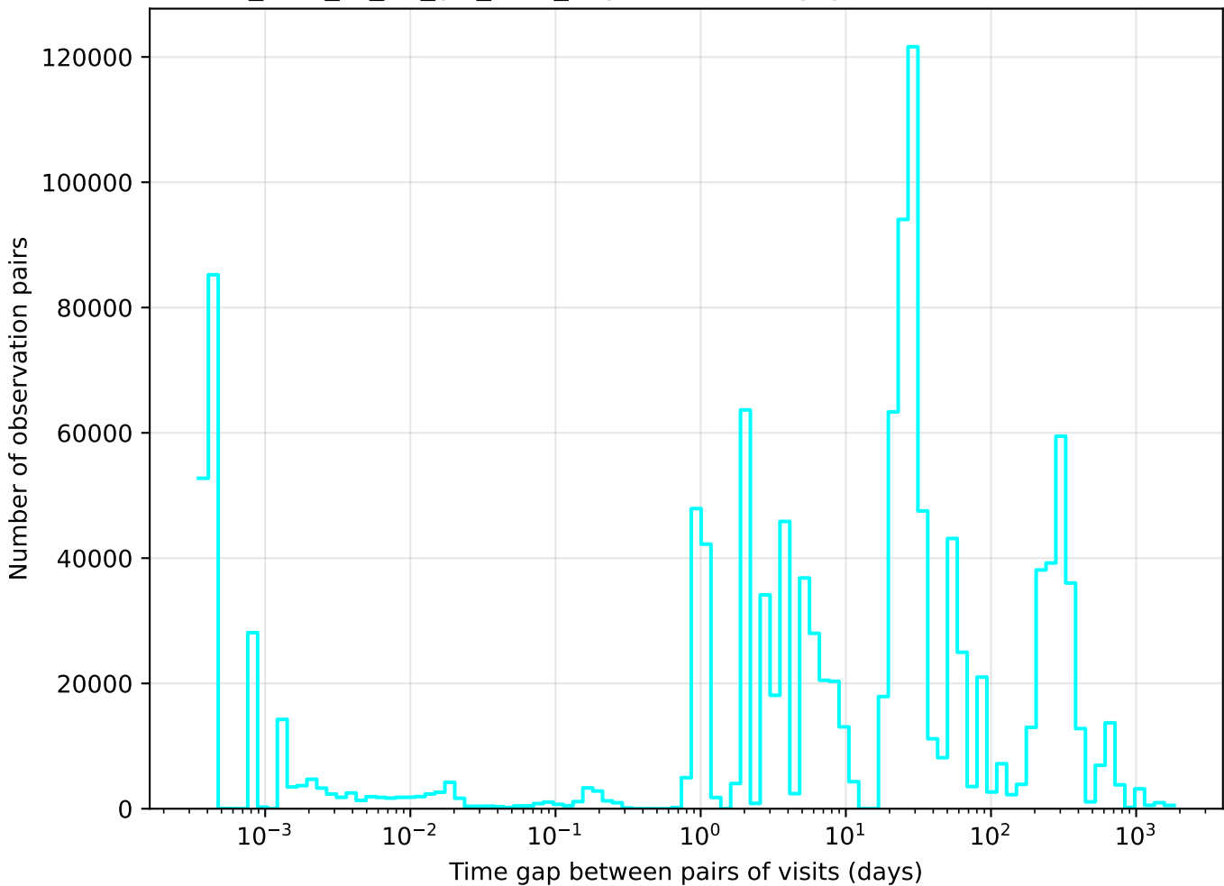
too_elab_r8_d3_giz_v3.4_10yrs u band: Tgaps observationStartMJD
