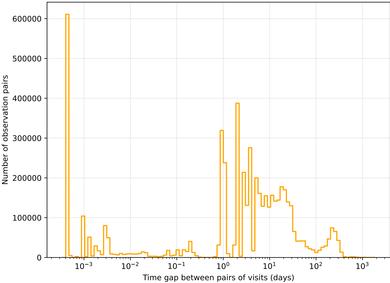
too_elab_r8_d3_giz_v3.4_10yrs r band: Tgaps observationStartMJD
