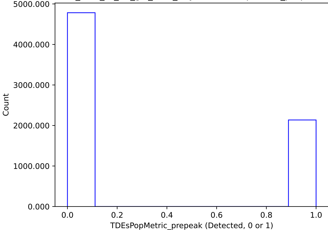
too_elab_r8_d3_giz_v3.4_10yrs : TDEsPopMetric_prepeak
