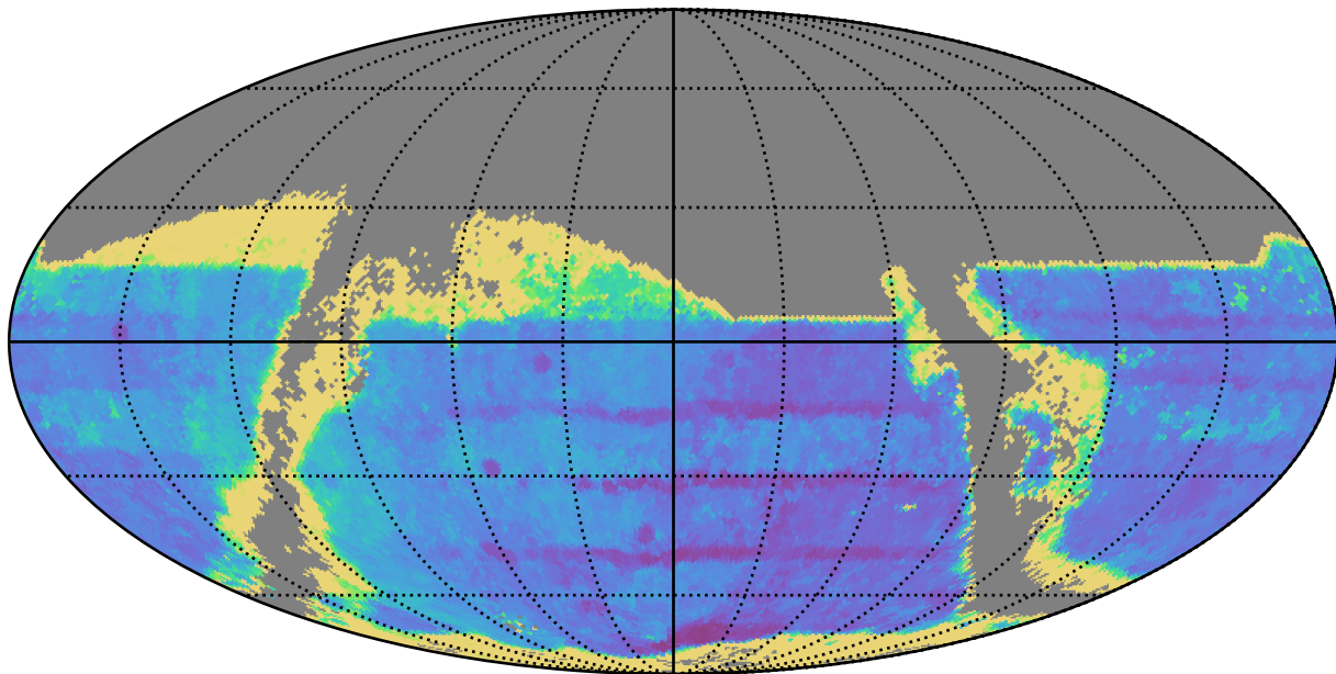
too_elab_r8_d3_giz_v3.4_10yrs : TDC_accuracy
