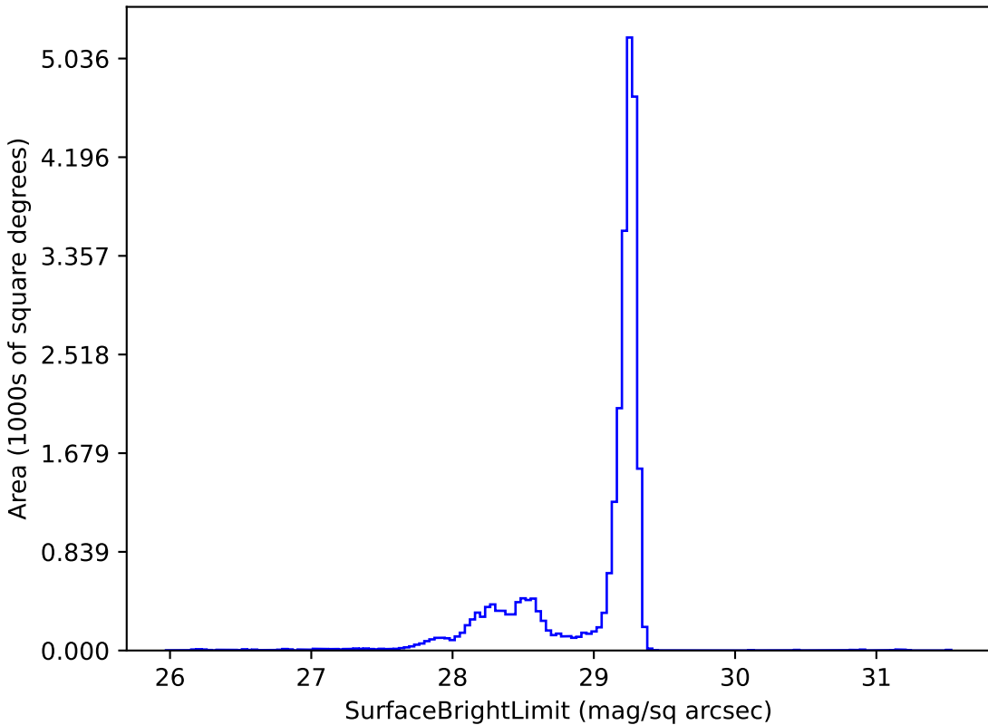
too_elab_r8_d3_giz_v3.4_10yrs z: SurfaceBrightLimit
