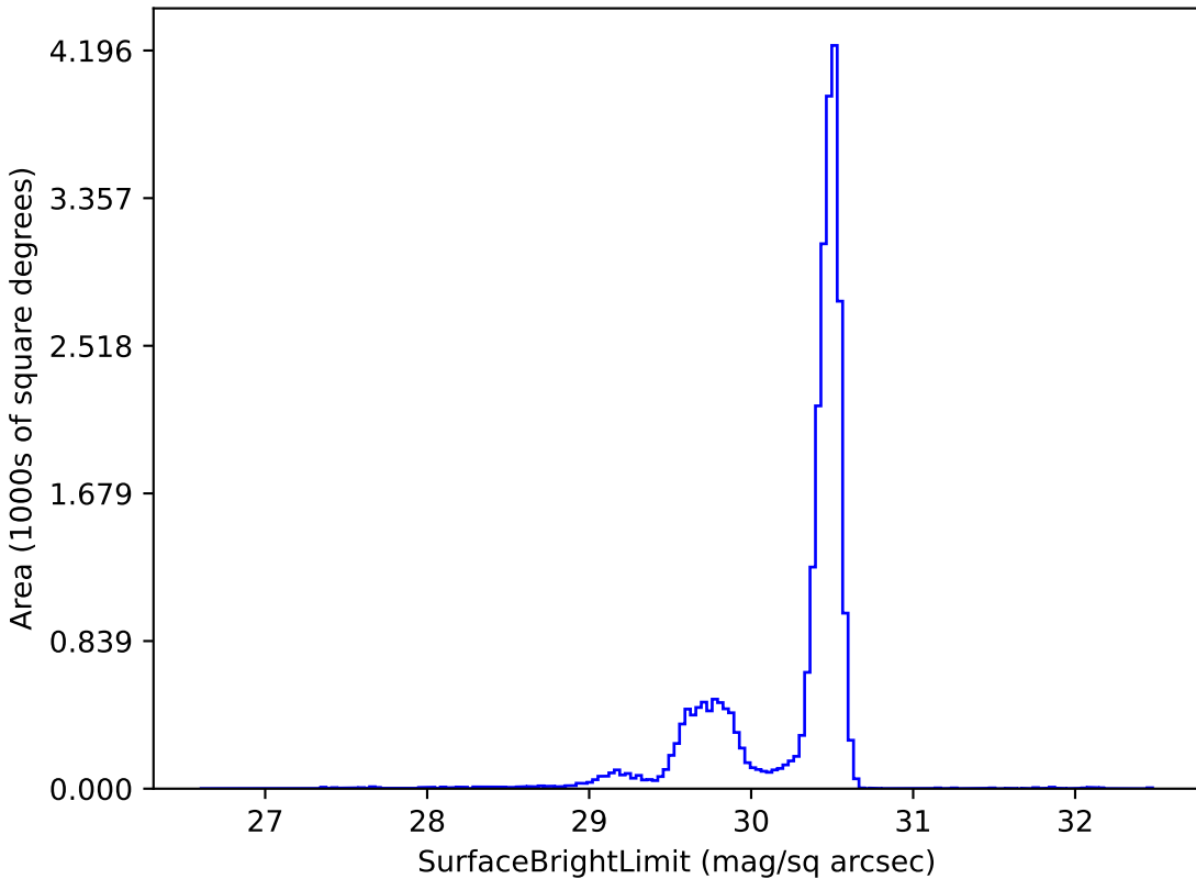
too_elab_r8_d3_giz_v3.4_10yrs r: SurfaceBrightLimit
