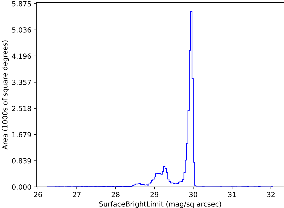
too_elab_r8_d3_giz_v3.4_10yrs i: SurfaceBrightLimit
