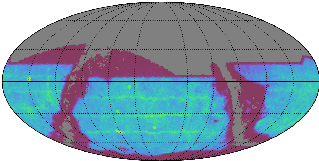
too_elab_r8_d3_giz_v3.4_10yrs : SNSLMetric
