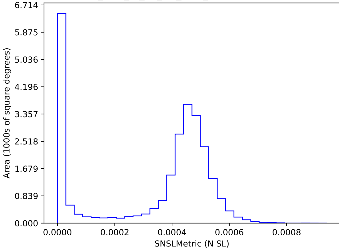
too_elab_r8_d3_giz_v3.4_10yrs : SNSLMetric
