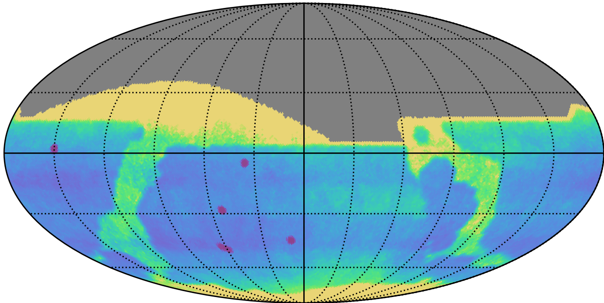
too_elab_r8_d3_giz_v3.4_10yrs : Proper Motion Uncert @ 24.0
