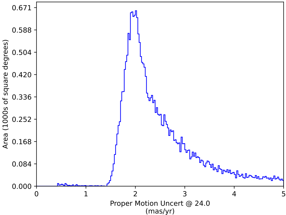
too_elab_r8_d3_giz_v3.4_10yrs : Proper Motion Uncert @ 24.0
