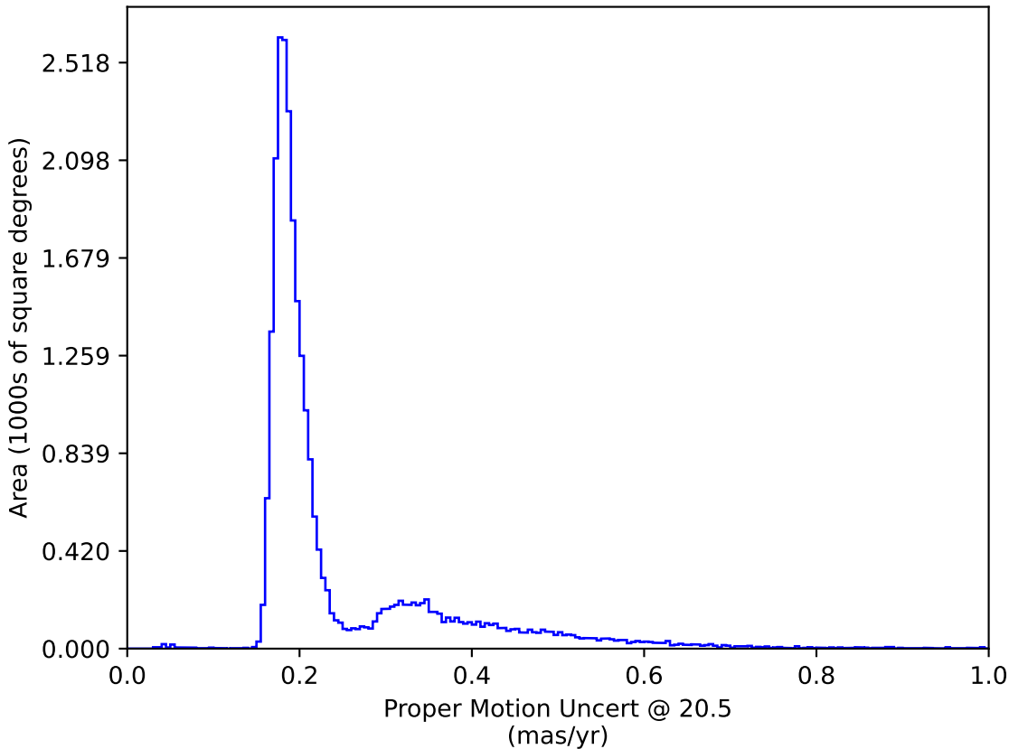
too_elab_r8_d3_giz_v3.4_10yrs : Proper Motion Uncert @ 20.5
