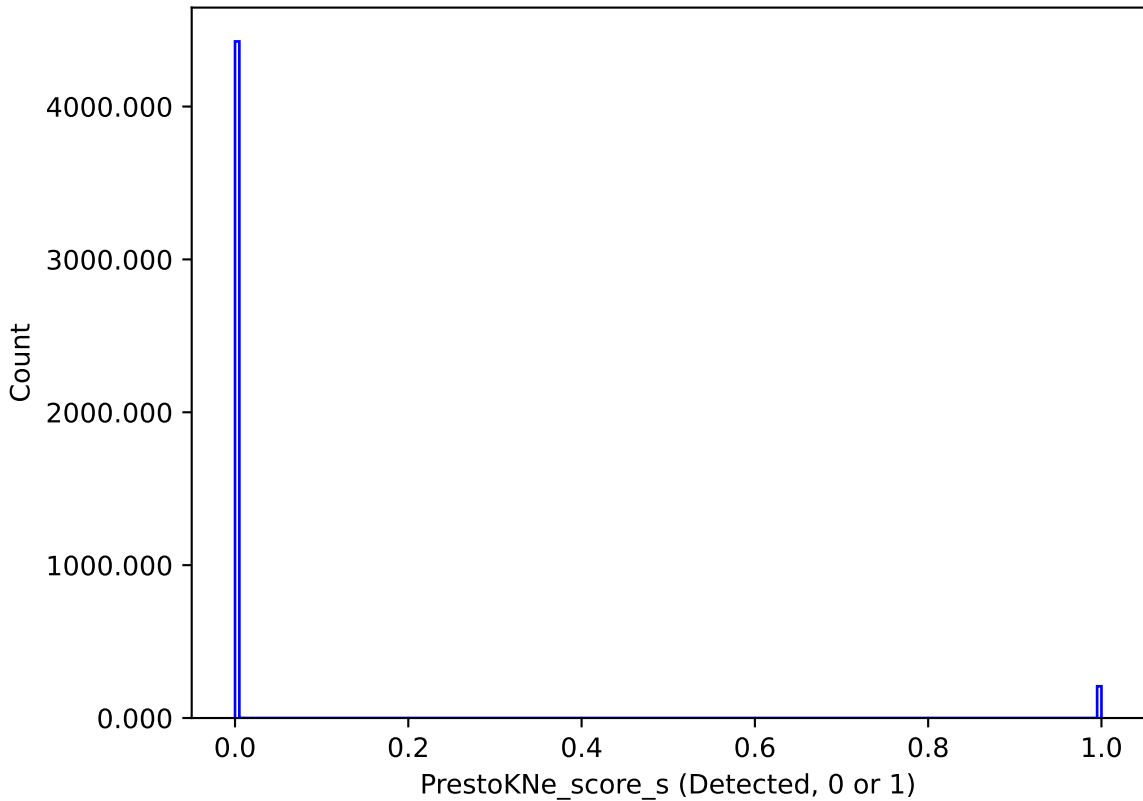
too_elab_r8_d3_giz_v3.4_10yrs : PrestoKNe_score_s
