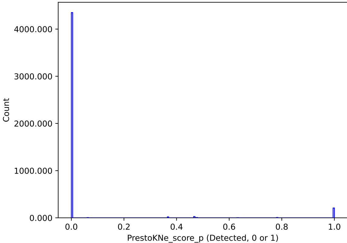
too_elab_r8_d3_giz_v3.4_10yrs : PrestoKNe_score_p
