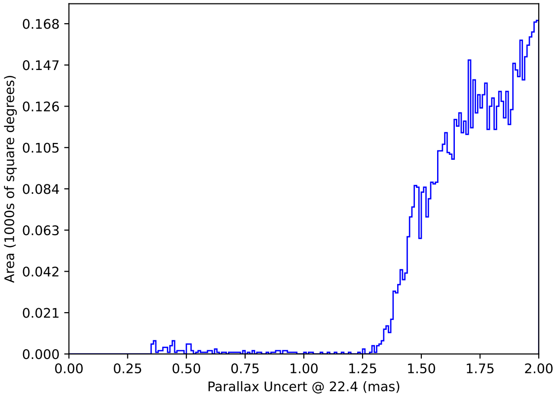
too_elab_r8_d3_giz_v3.4_10yrs : Parallax Uncert @ 22.4
