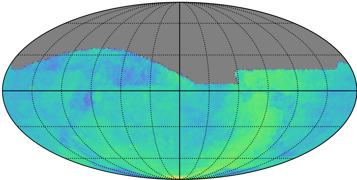
too_elab_r8_d3_giz_v3.4_10yrs : Parallax Coverage @ 24.0
