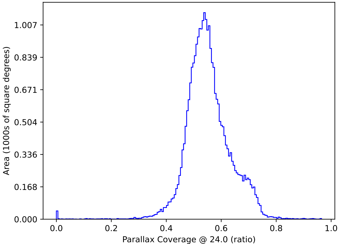
too_elab_r8_d3_giz_v3.4_10yrs : Parallax Coverage @ 24.0
