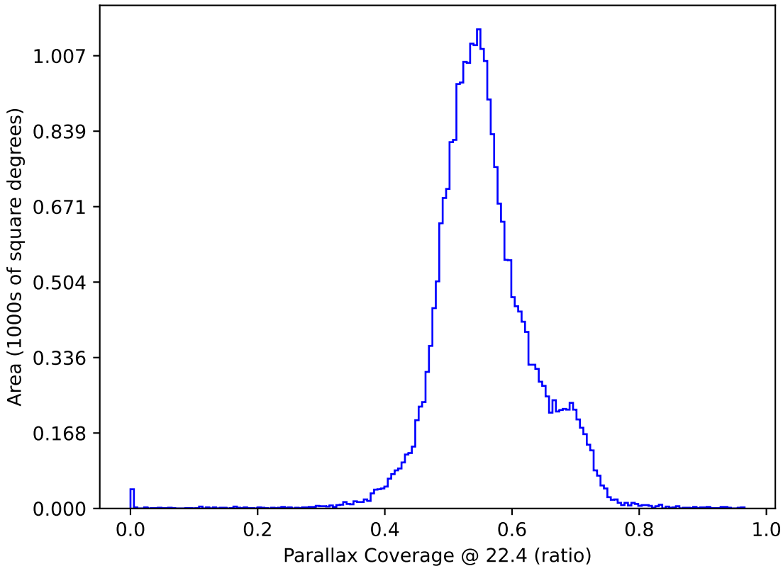
too_elab_r8_d3_giz_v3.4_10yrs : Parallax Coverage @ 22.4
