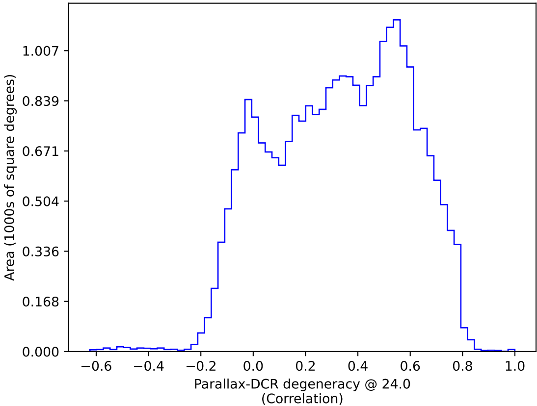
too_elab_r8_d3_giz_v3.4_10yrs : Parallax-DCR degeneracy @ 24.0
