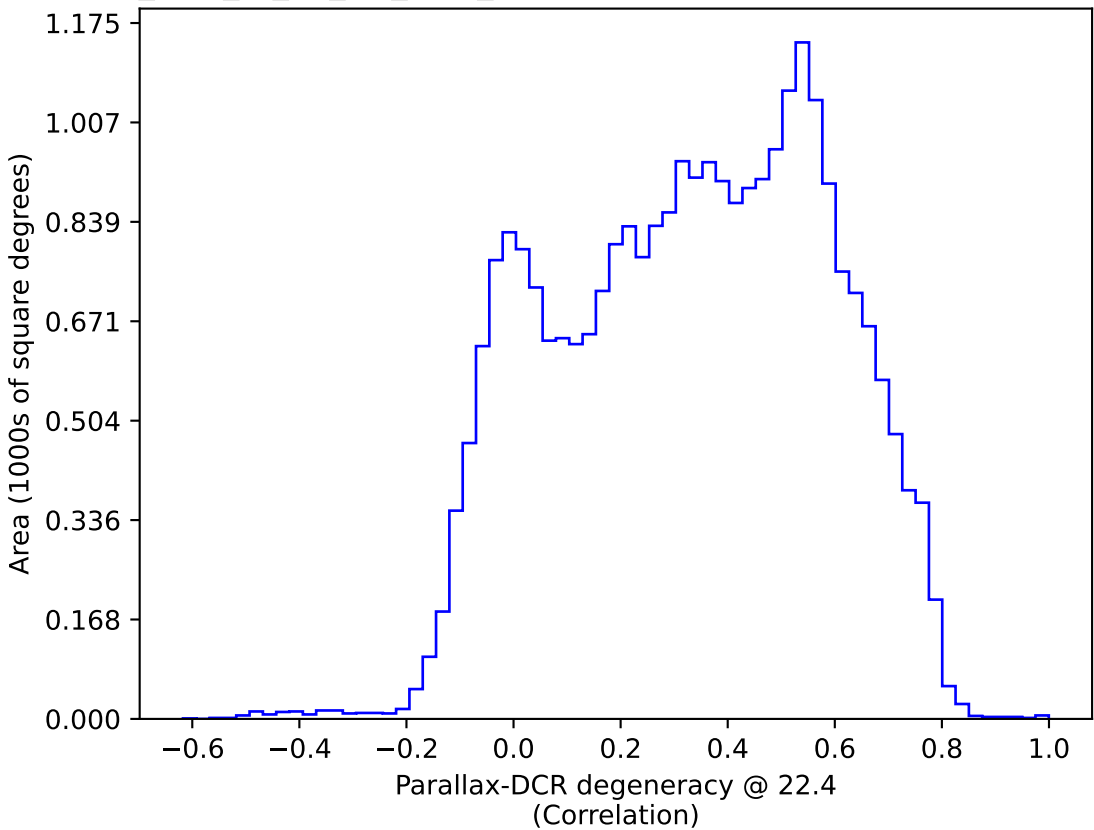
too_elab_r8_d3_giz_v3.4_10yrs : Parallax-DCR degeneracy @ 22.4
