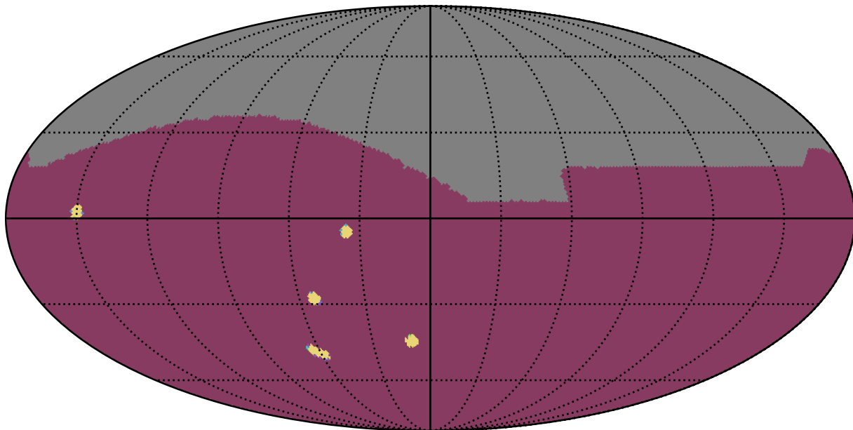
too_elab_r8_d3_giz_v3.4_10yrs : NumberOfQuickRevisits
