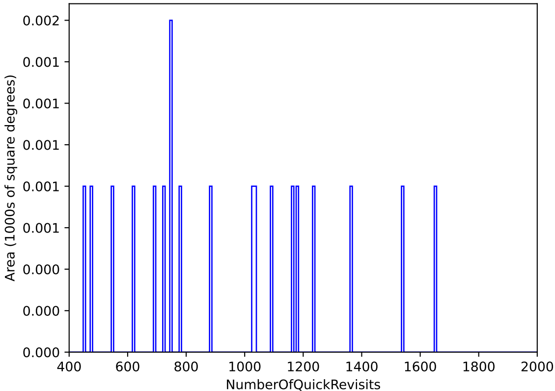
too_elab_r8_d3_giz_v3.4_10yrs : NumberOfQuickRevisits
