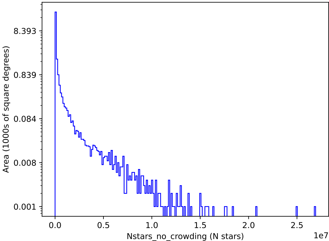
too_elab_r8_d3_giz_v3.4_10yrs z: Nstars_no_crowding
