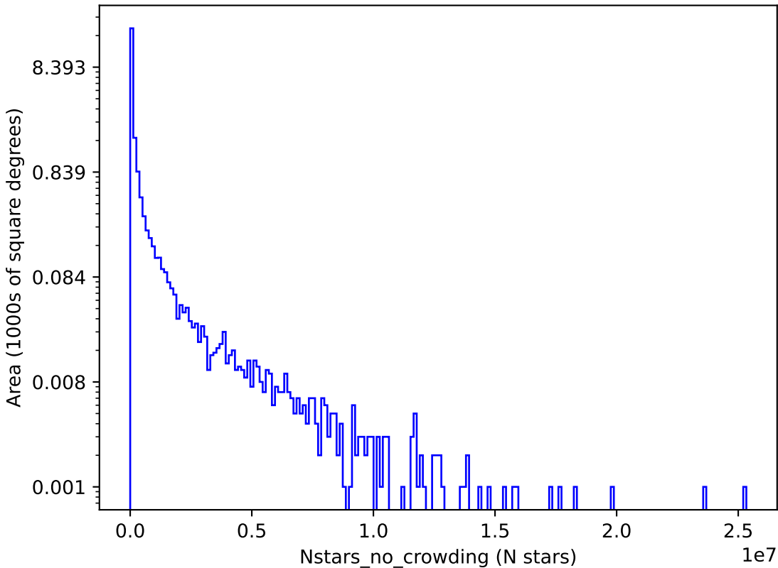
too_elab_r8_d3_giz_v3.4_10yrs y: Nstars_no_crowding
