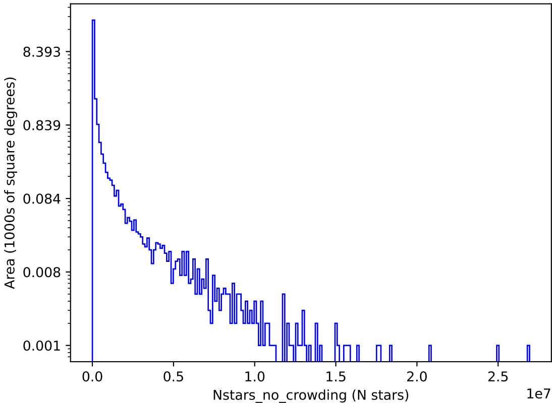
too_elab_r8_d3_giz_v3.4_10yrs i: Nstars_no_crowding
