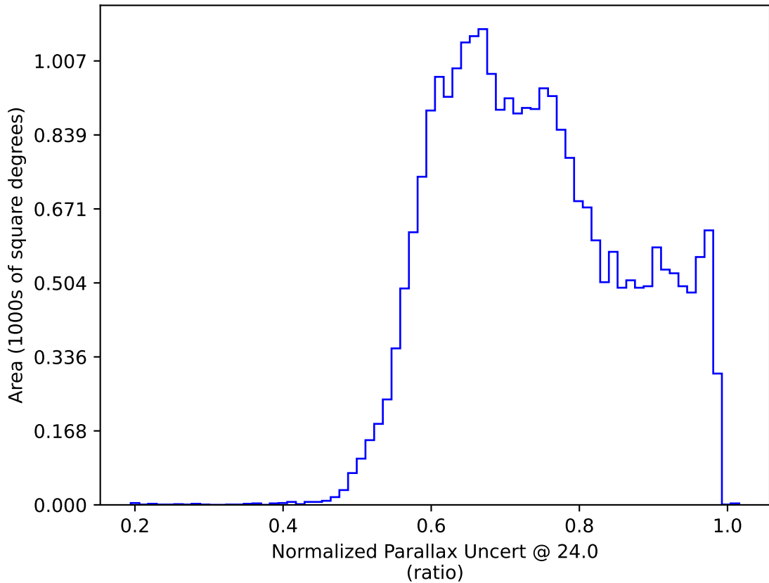
too_elab_r8_d3_giz_v3.4_10yrs : Normalized Parallax Uncert @ 24.0
