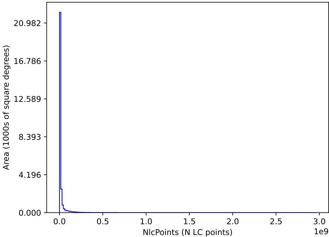
too_elab_r8_d3_giz_v3.4_10yrs : NlcPoints
