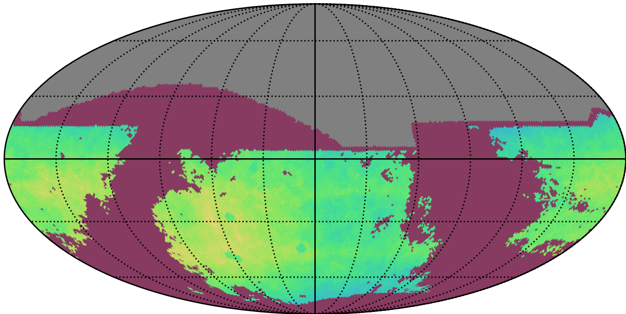
too_elab_r8_d3_giz_v3.4_10yrs i: NgalScale
