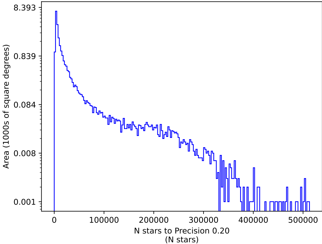
too_elab_r8_d3_giz_v3.4_10yrs u: N stars to Precision 0.20
