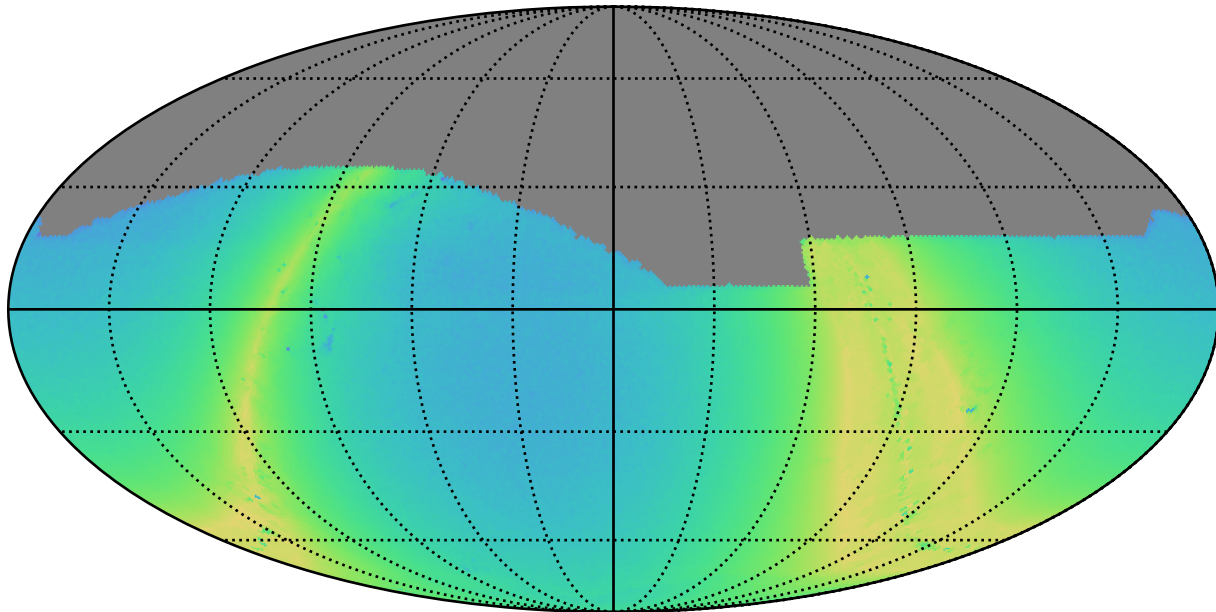
too_elab_r8_d3_giz_v3.4_10yrs i: N stars to Precision 0.20
