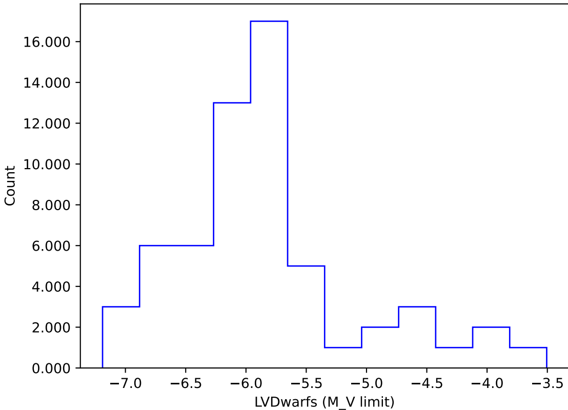
too_elab_r8_d3_giz_v3.4_10yrs gi: LVDwarfs
