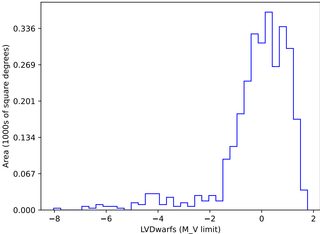
too_elab_r8_d3_giz_v3.4_10yrs gi SCP: LVDwarfs
