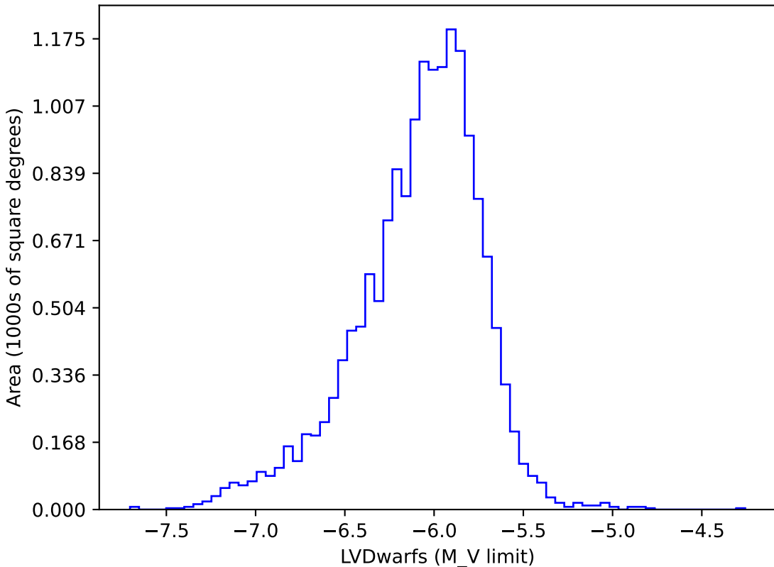
too_elab_r8_d3_giz_v3.4_10yrs gi: LVDwarfs
