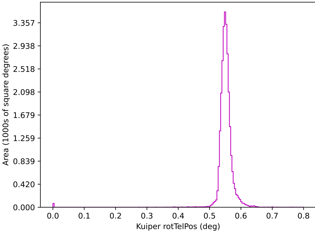
too_elab_r8_d3_giz_v3.4_10yrs z: Kuiper rotTelPos
