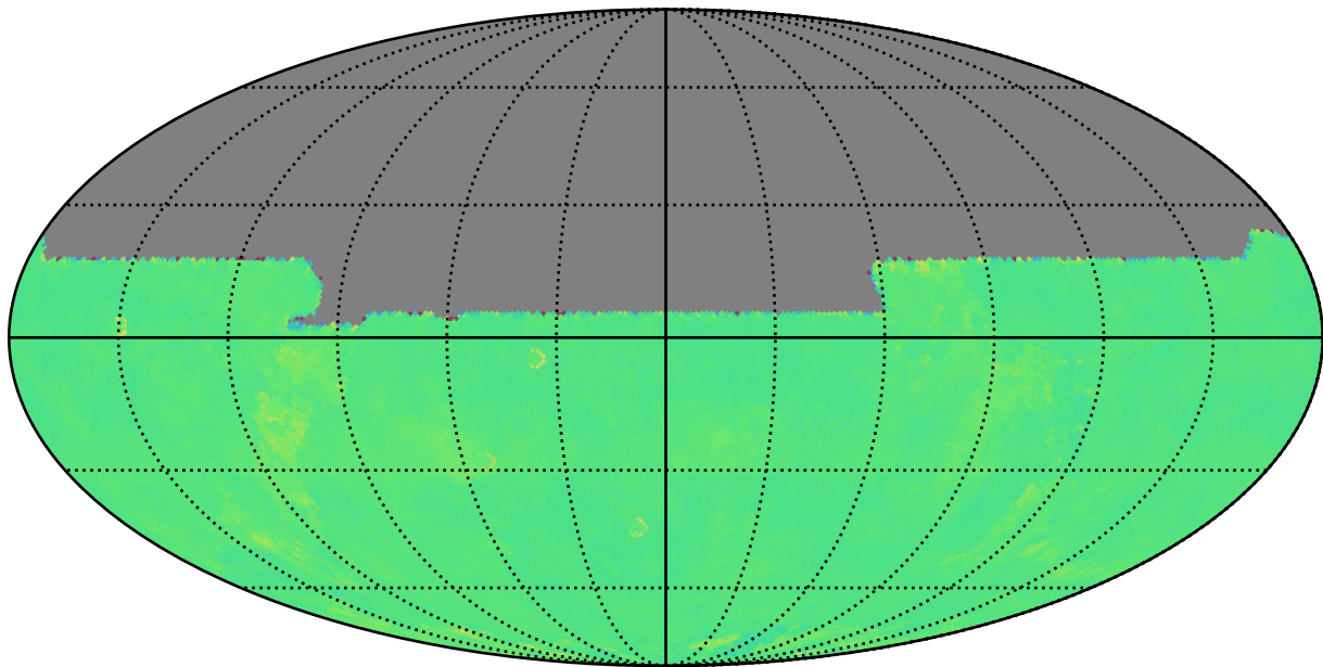
too_elab_r8_d3_giz_v3.4_10yrs y: Kuiper rotTelPos
