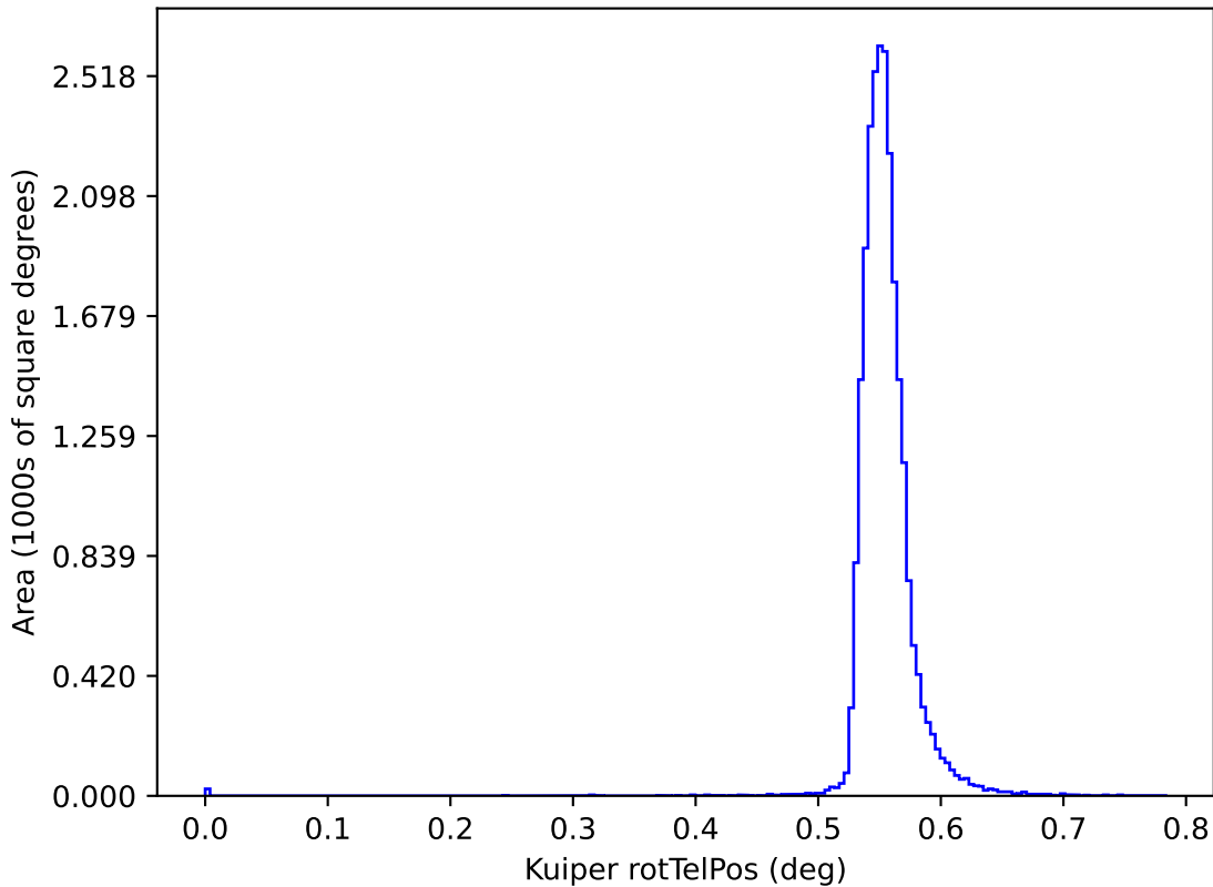
too_elab_r8_d3_giz_v3.4_10yrs y: Kuiper rotTelPos
