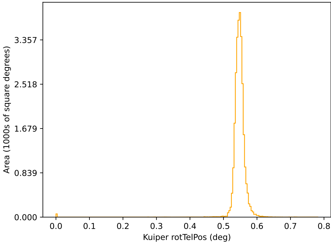
too_elab_r8_d3_giz_v3.4_10yrs r: Kuiper rotTelPos
