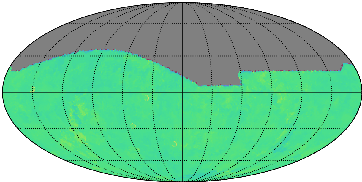
too_elab_r8_d3_giz_v3.4_10yrs g: Kuiper rotTelPos
