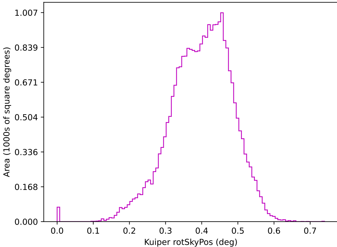
too_elab_r8_d3_giz_v3.4_10yrs z: Kuiper rotSkyPos
