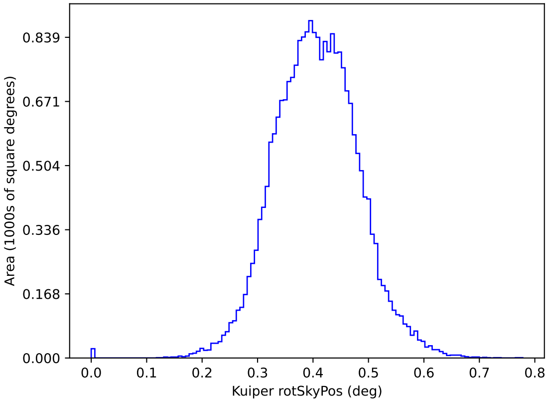
too_elab_r8_d3_giz_v3.4_10yrs y: Kuiper rotSkyPos
