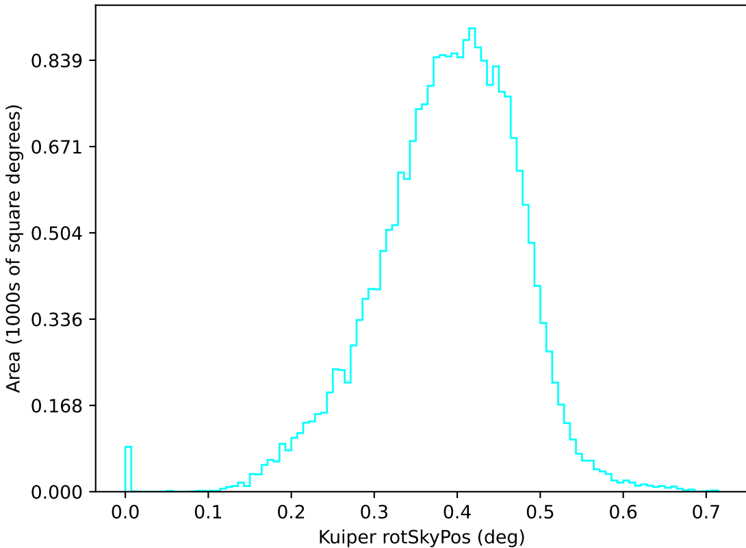
too_elab_r8_d3_giz_v3.4_10yrs u: Kuiper rotSkyPos
