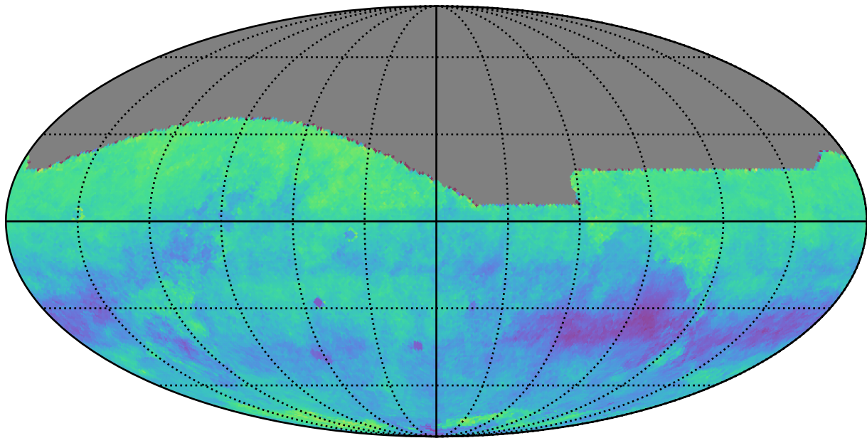
too_elab_r8_d3_giz_v3.4_10yrs r: Kuiper rotSkyPos
