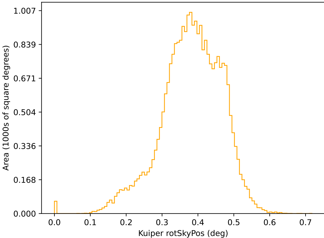
too_elab_r8_d3_giz_v3.4_10yrs r: Kuiper rotSkyPos
