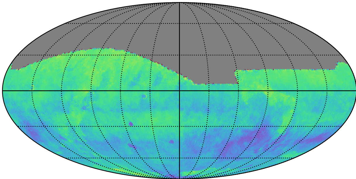
too_elab_r8_d3_giz_v3.4_10yrs i: Kuiper rotSkyPos
